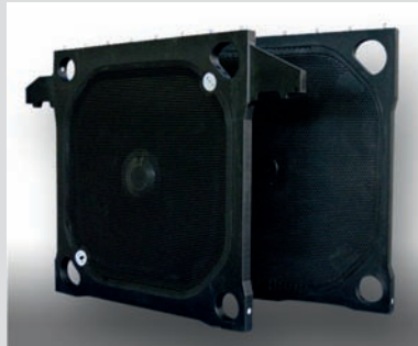
High pressure membrane plate up to 50 bar 1,5m x 1,5m
